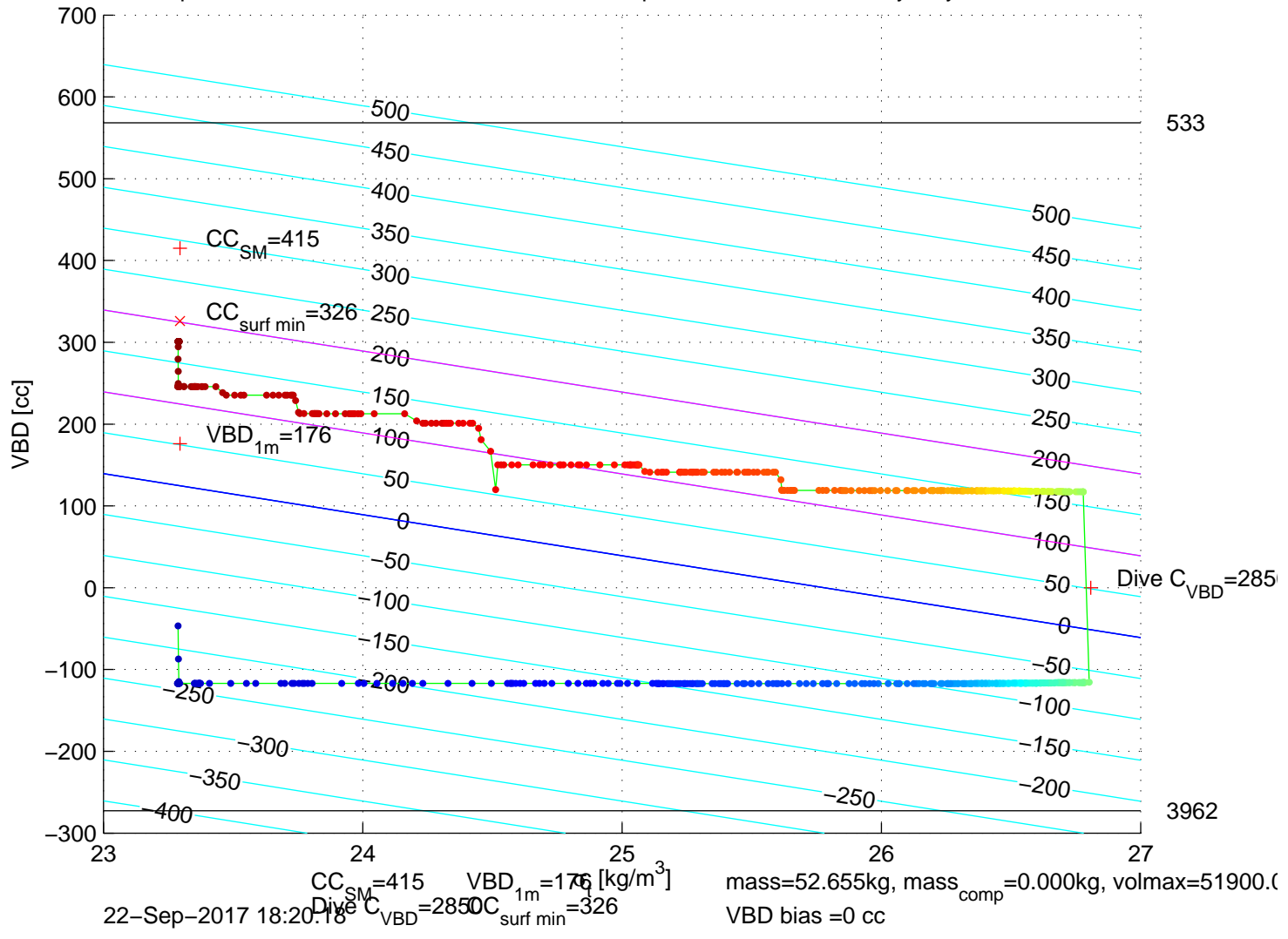
p6350529: SG635 Mission 7 Jul 2017 22-Sep-2017 19:43:10Z – buoyancy contoured
