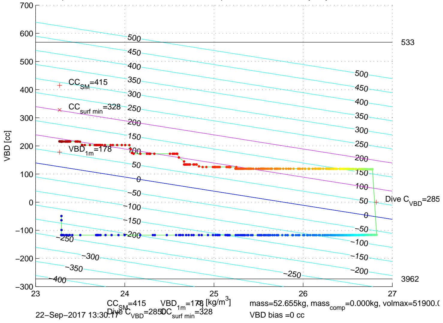
p6350527: SG635 Mission 7 Jul 2017 22-Sep-2017 15:13:57Z – buoyancy contoured
