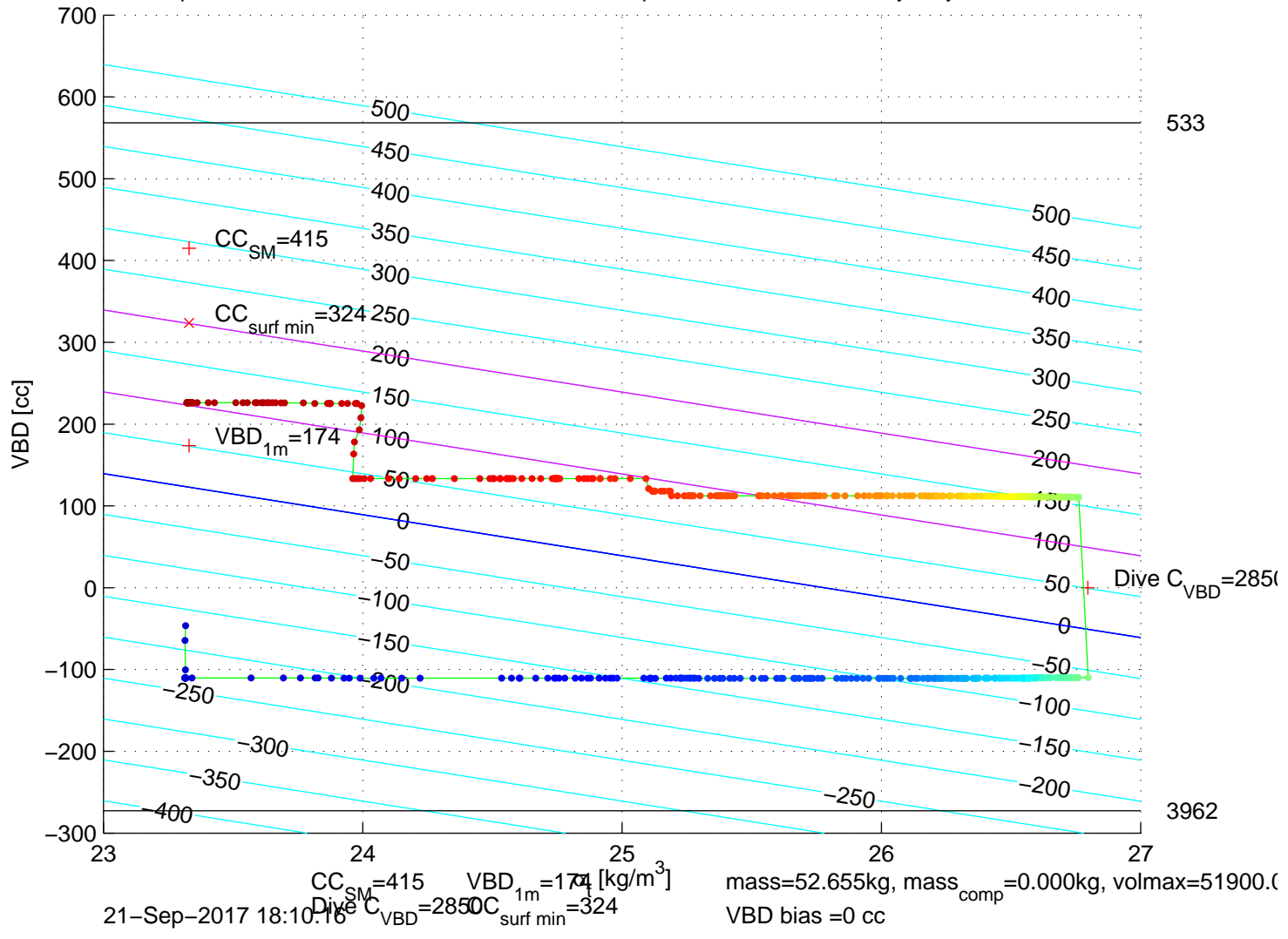
p6350518: SG635 Mission 7 Jul 2017 21-Sep-2017 19:54:27Z - buoyancy contoured
