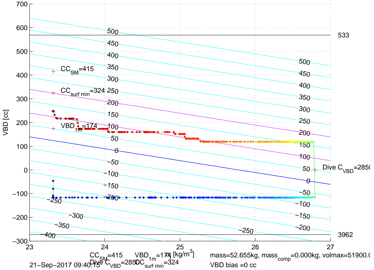
p6350514: SG635 Mission 7 Jul 2017 21-Sep-2017 11:15:06Z – buoyancy contoured
