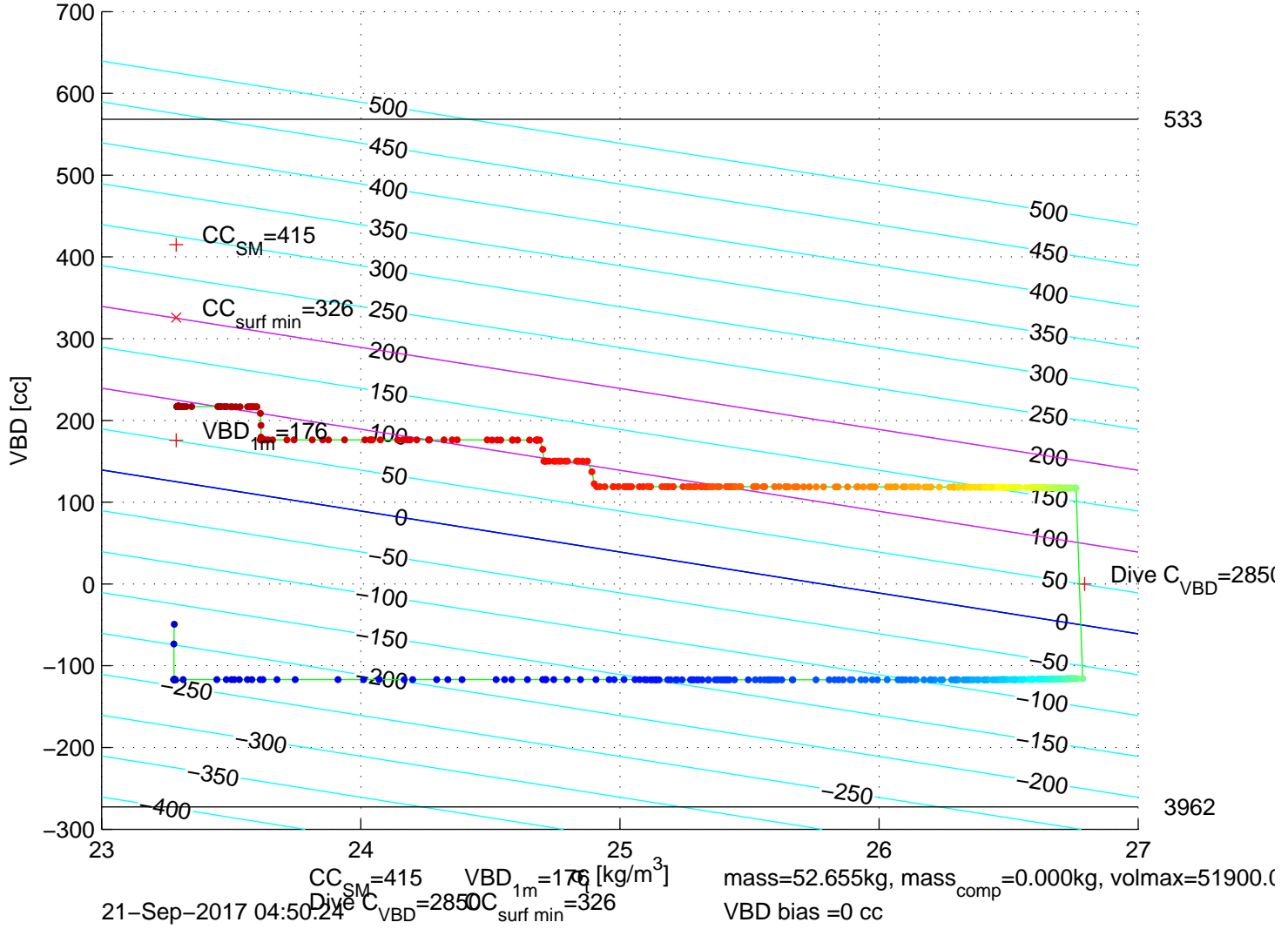
p6350512: SG635 Mission 7 Jul 2017 21-Sep-2017 06:40:49Z – buoyancy contoured
