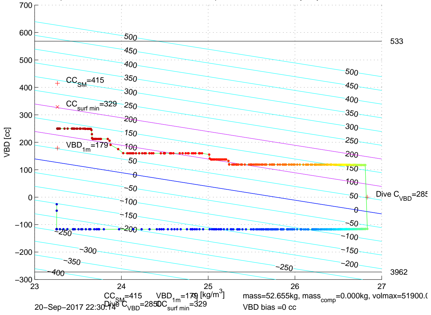
p6350509: SG635 Mission 7 Jul 2017 21-Sep-2017 00:11:28Z - buoyancy contoured
