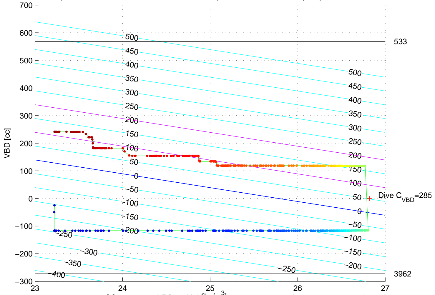
p6350506: SG635 Mission 7 Jul 2017 20-Sep-2017 17:56:34Z – buoyancy contoured
