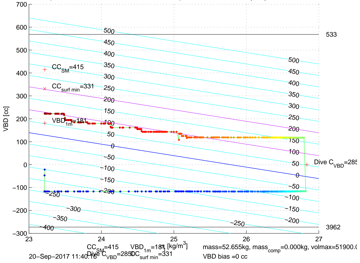
p6350504: SG635 Mission 7 Jul 2017 20-Sep-2017 13:31:15Z – buoyancy contoured
