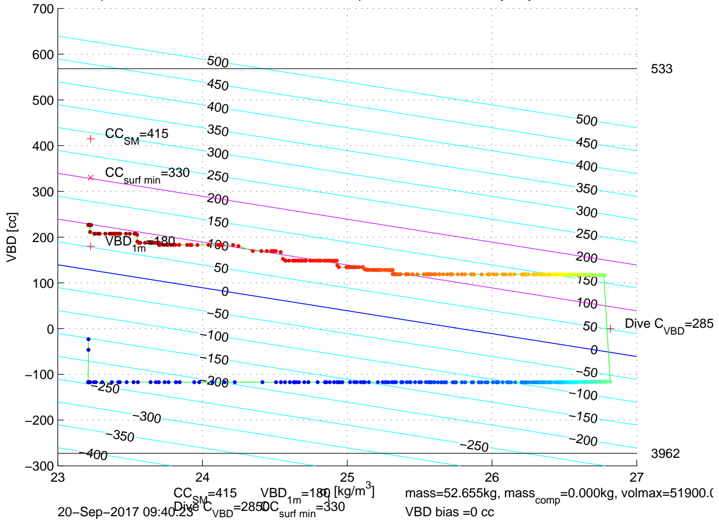
p6350503: SG635 Mission 7 Jul 2017 20-Sep-2017 11:25:30Z – buoyancy contoured
