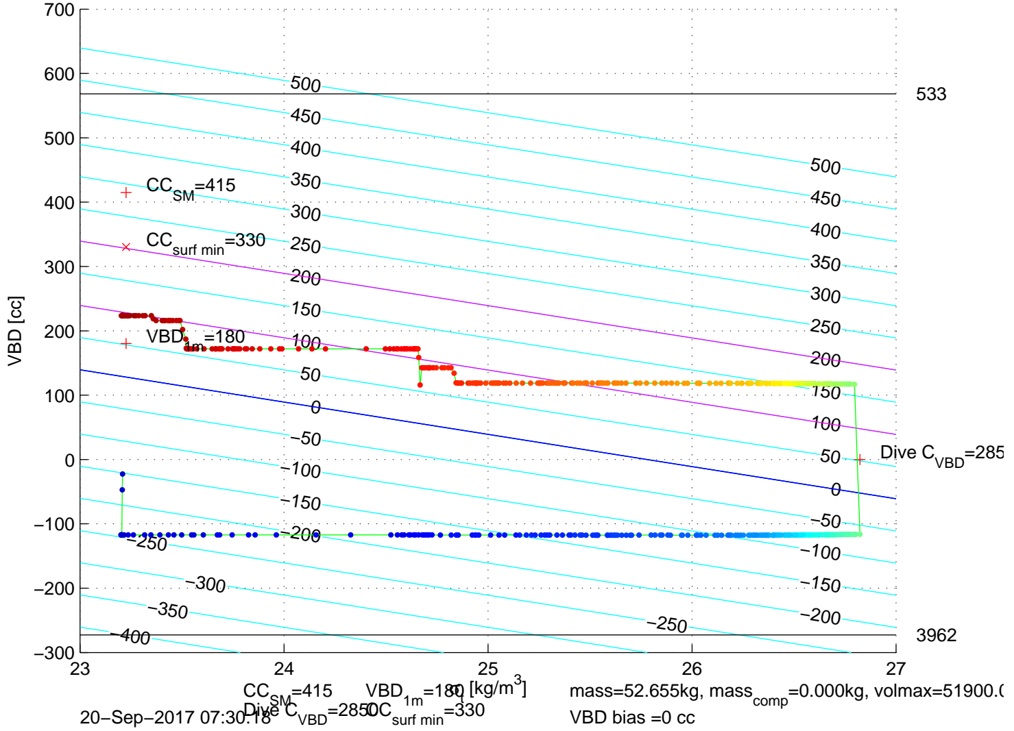
p6350502: SG635 Mission 7 Jul 2017 20-Sep-2017 09:17:14Z – buoyancy contoured
