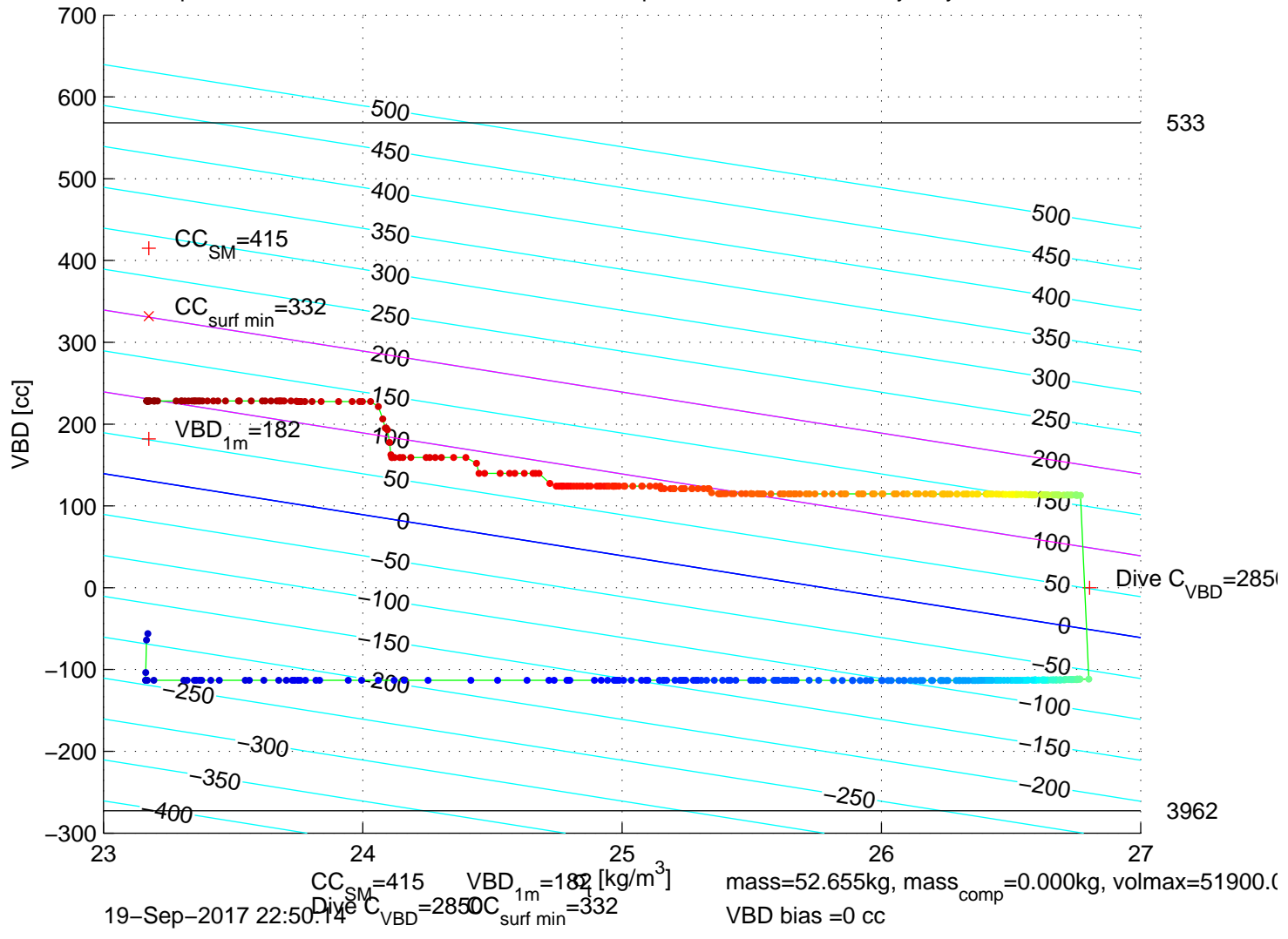
p6350498: SG635 Mission 7 Jul 2017 20-Sep-2017 00:35:44Z – buoyancy contoured
