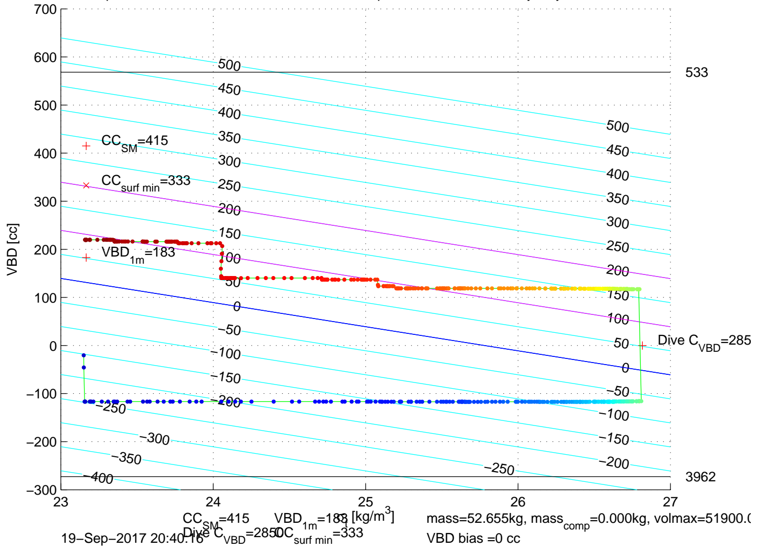
p6350497: SG635 Mission 7 Jul 2017 19-Sep-2017 22:29:52Z – buoyancy contoured
