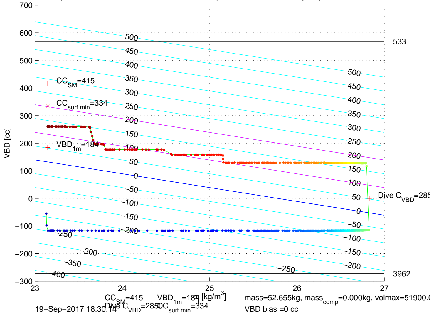
p6350496: SG635 Mission 7 Jul 2017 19-Sep-2017 20:08:52Z – buoyancy contoured
