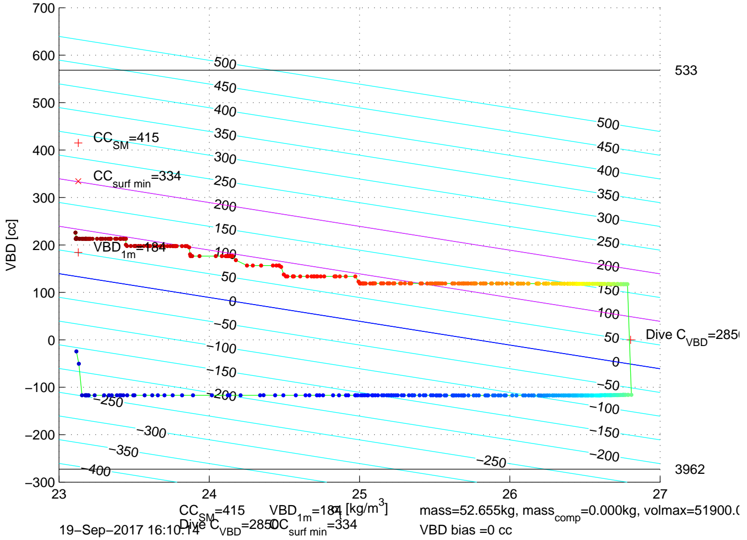
p6350495: SG635 Mission 7 Jul 2017 19-Sep-2017 18:01:25Z – buoyancy contoured
