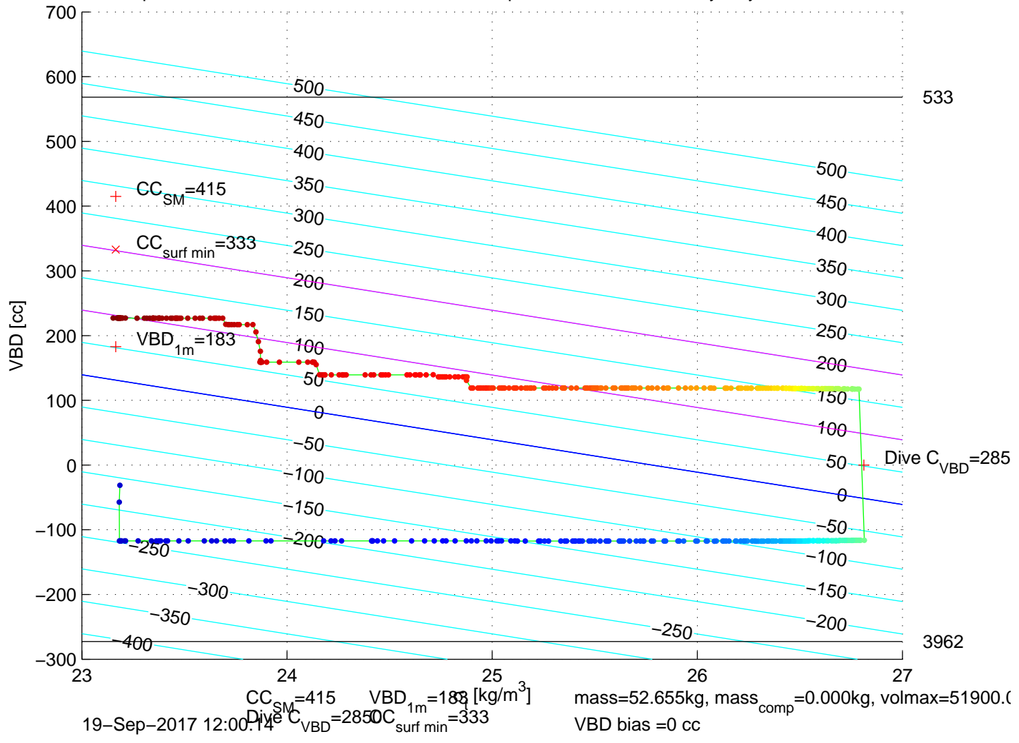
p6350493: SG635 Mission 7 Jul 2017 19-Sep-2017 13:47:33Z – buoyancy contoured
