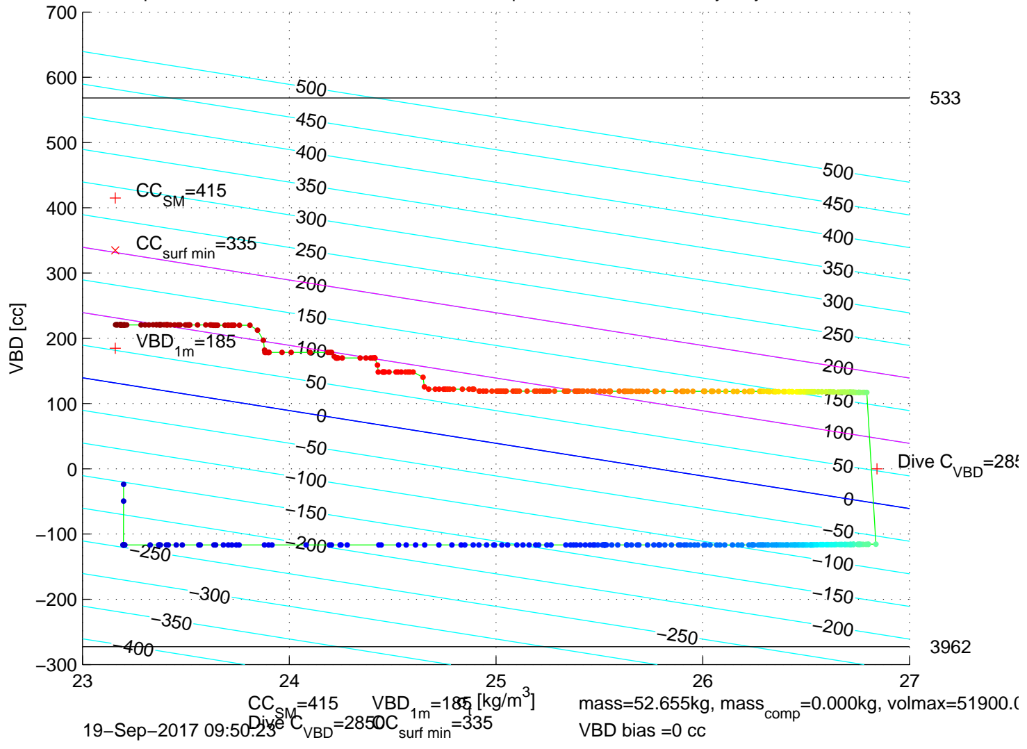
p6350492: SG635 Mission 7 Jul 2017 19-Sep-2017 11:41:46Z – buoyancy contoured
