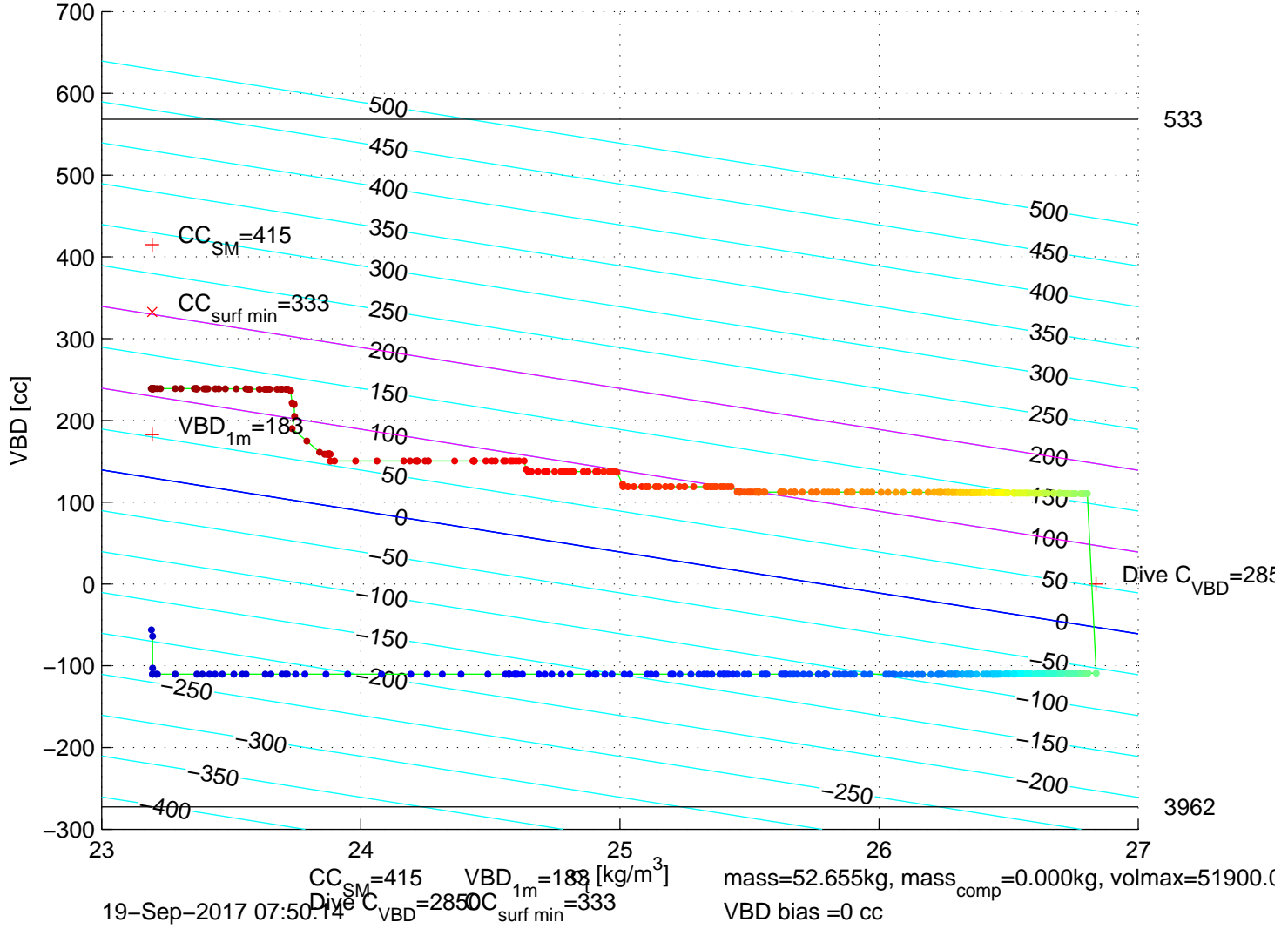
p6350491: SG635 Mission 7 Jul 2017 19-Sep-2017 09:31:52Z – buoyancy contoured
