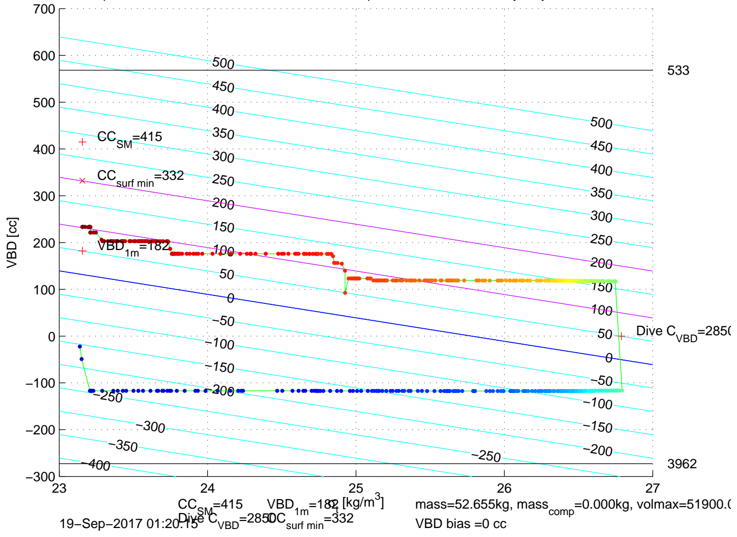
p6350488: SG635 Mission 7 Jul 2017 19-Sep-2017 03:15:35Z – buoyancy contoured
