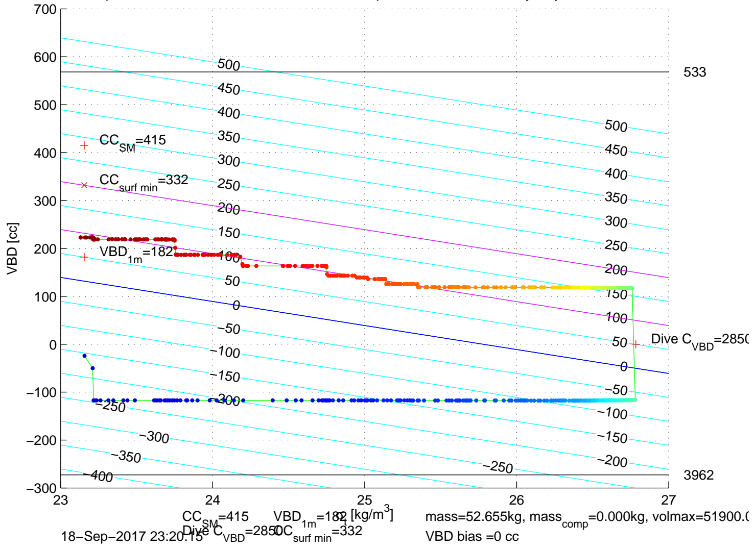
p6350487: SG635 Mission 7 Jul 2017 19-Sep-2017 01:07:26Z – buoyancy contoured
