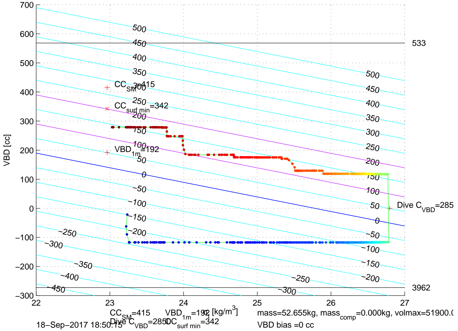
p6350485: SG635 Mission 7 Jul 2017 18-Sep-2017 20:14:34Z – buoyancy contoured
