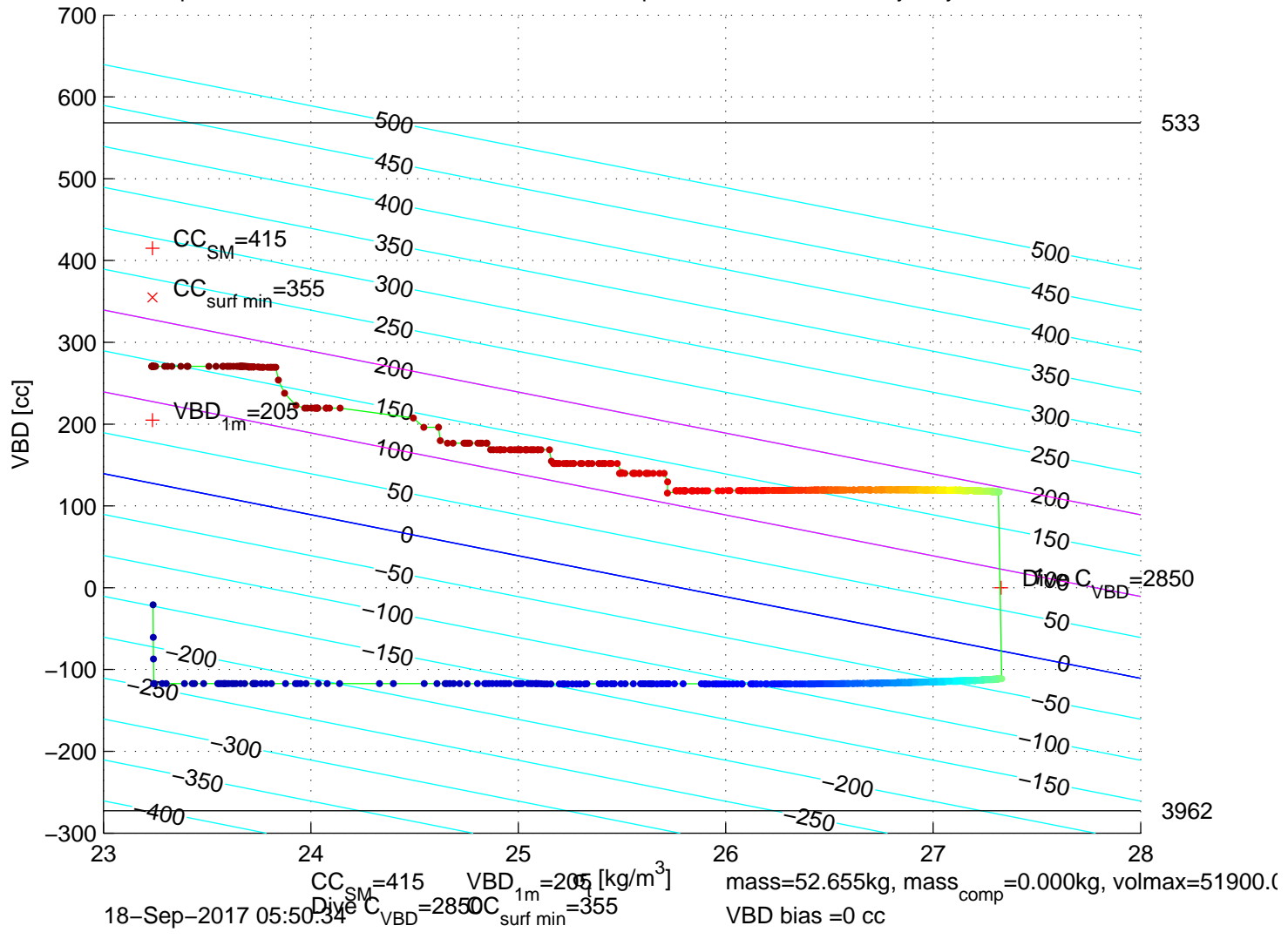
p6350481: SG635 Mission 7 Jul 2017 18-Sep-2017 05:12:20Z – buoyancy contoured
