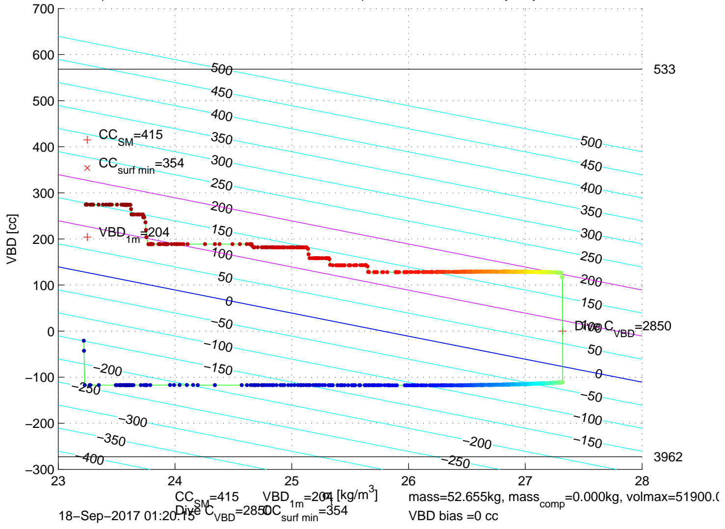
p6350480: SG635 Mission 7 Jul 2017 18-Sep-2017 00:46:29Z – buoyancy contoured
