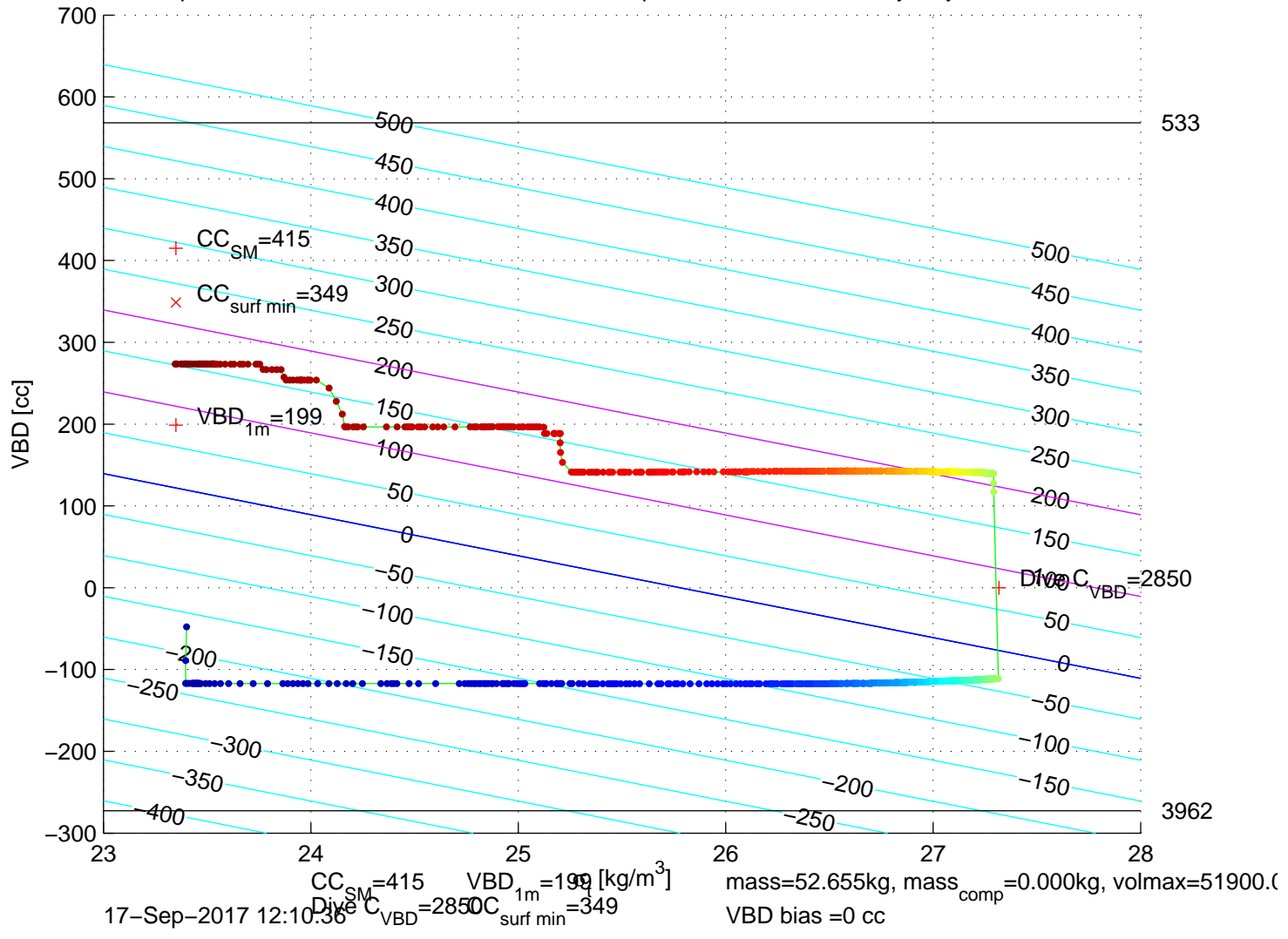
p6350477: SG635 Mission 7 Jul 2017 17-Sep-2017 11:50:12Z – buoyancy contoured
