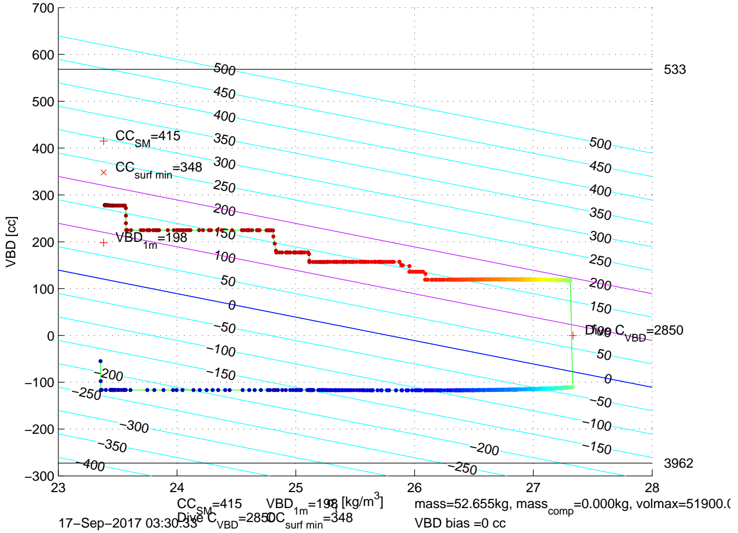
p6350475: SG635 Mission 7 Jul 2017 17-Sep-2017 02:59:53Z – buoyancy contoured
