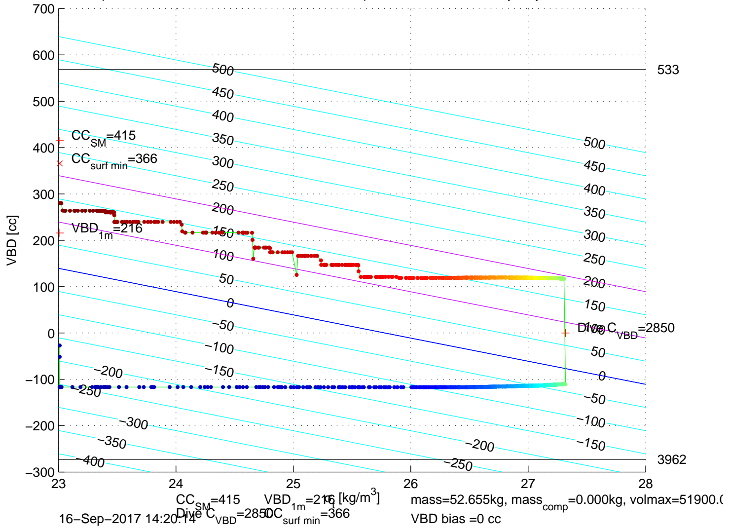
p6350472: SG635 Mission 7 Jul 2017 16-Sep-2017 13:47:04Z – buoyancy contoured
