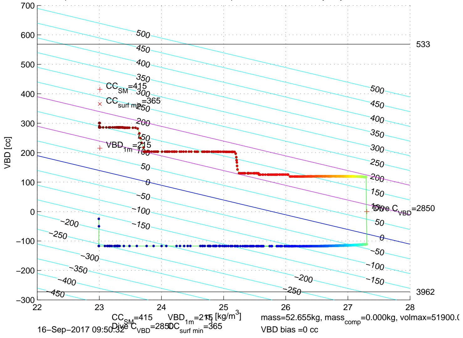
p6350471: SG635 Mission 7 Jul 2017 16-Sep-2017 09:18:26Z – buoyancy contoured
