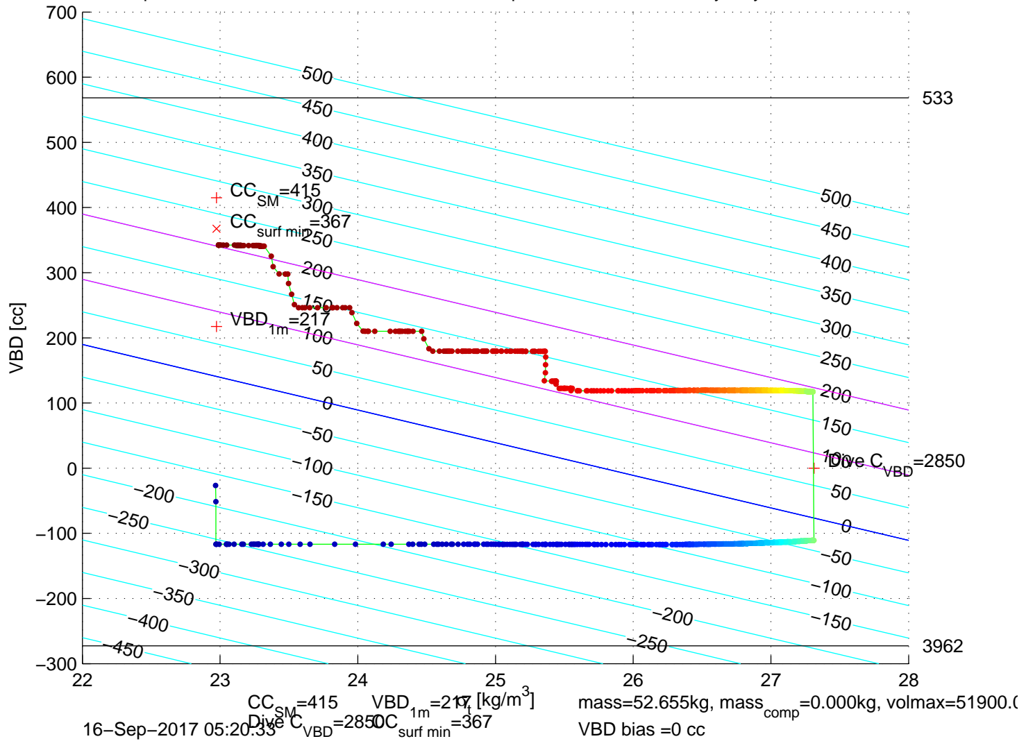
p6350470: SG635 Mission 7 Jul 2017 16-Sep-2017 04:56:00Z – buoyancy contoured
