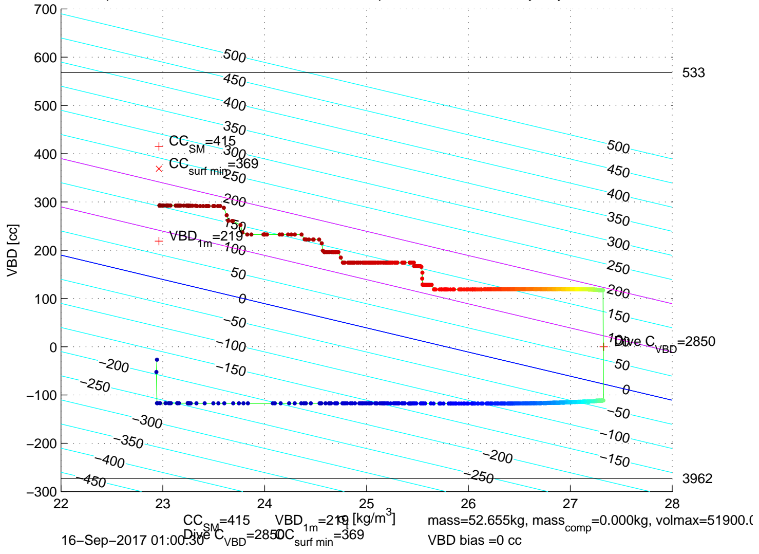
p6350469: SG635 Mission 7 Jul 2017 16-Sep-2017 00:30:26Z – buoyancy contoured
