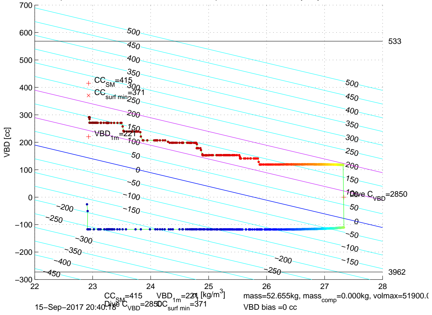
p6350468: SG635 Mission 7 Jul 2017 15-Sep-2017 19:59:34Z – buoyancy contoured
