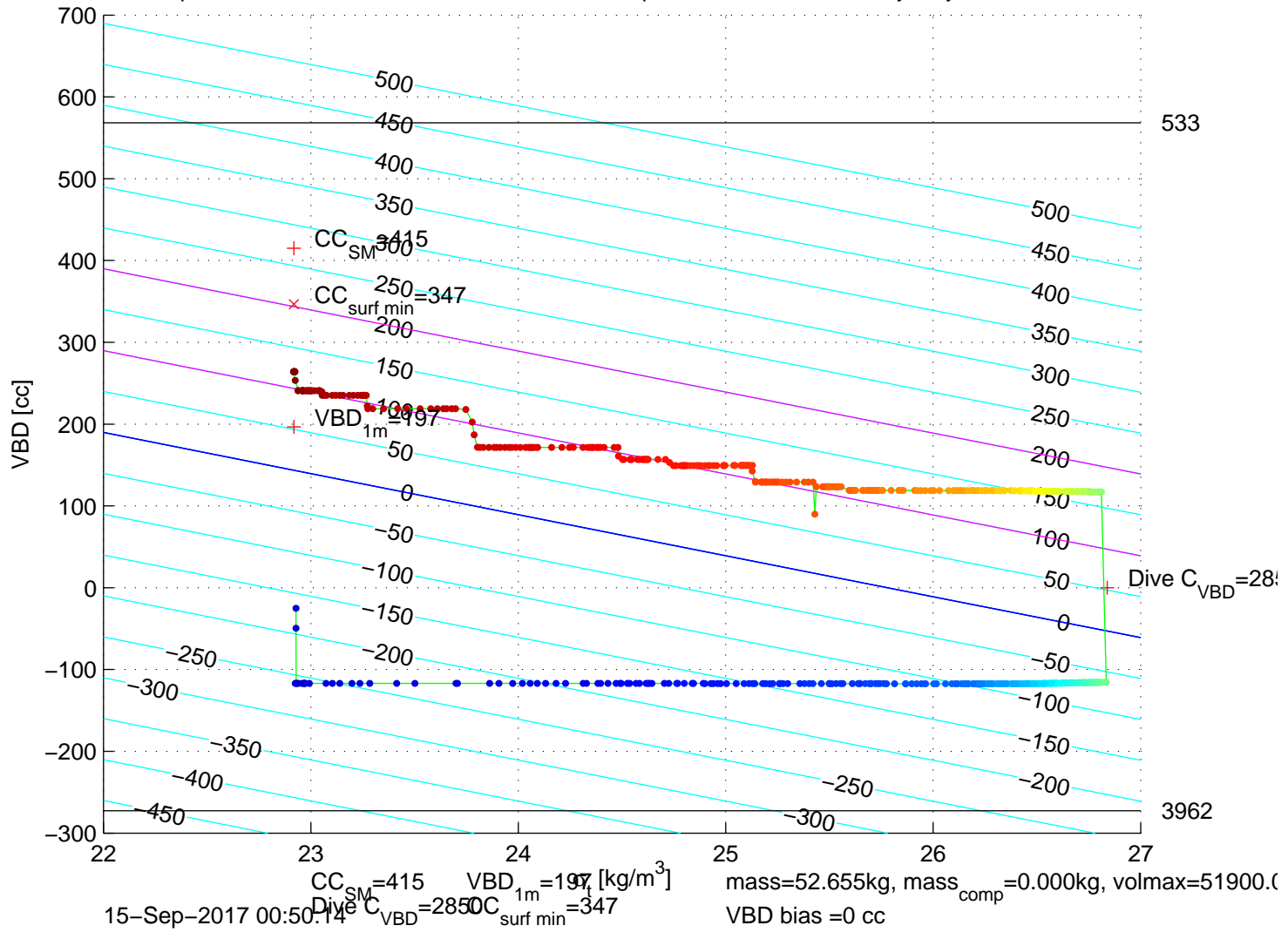
p6350461: SG635 Mission 7 Jul 2017 15-Sep-2017 02:28:30Z – buoyancy contoured
