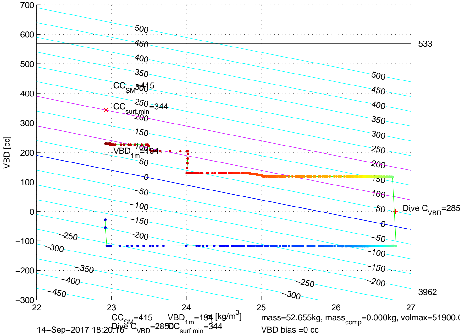
p6350458: SG635 Mission 7 Jul 2017 14-Sep-2017 20:09:18Z – buoyancy contoured
