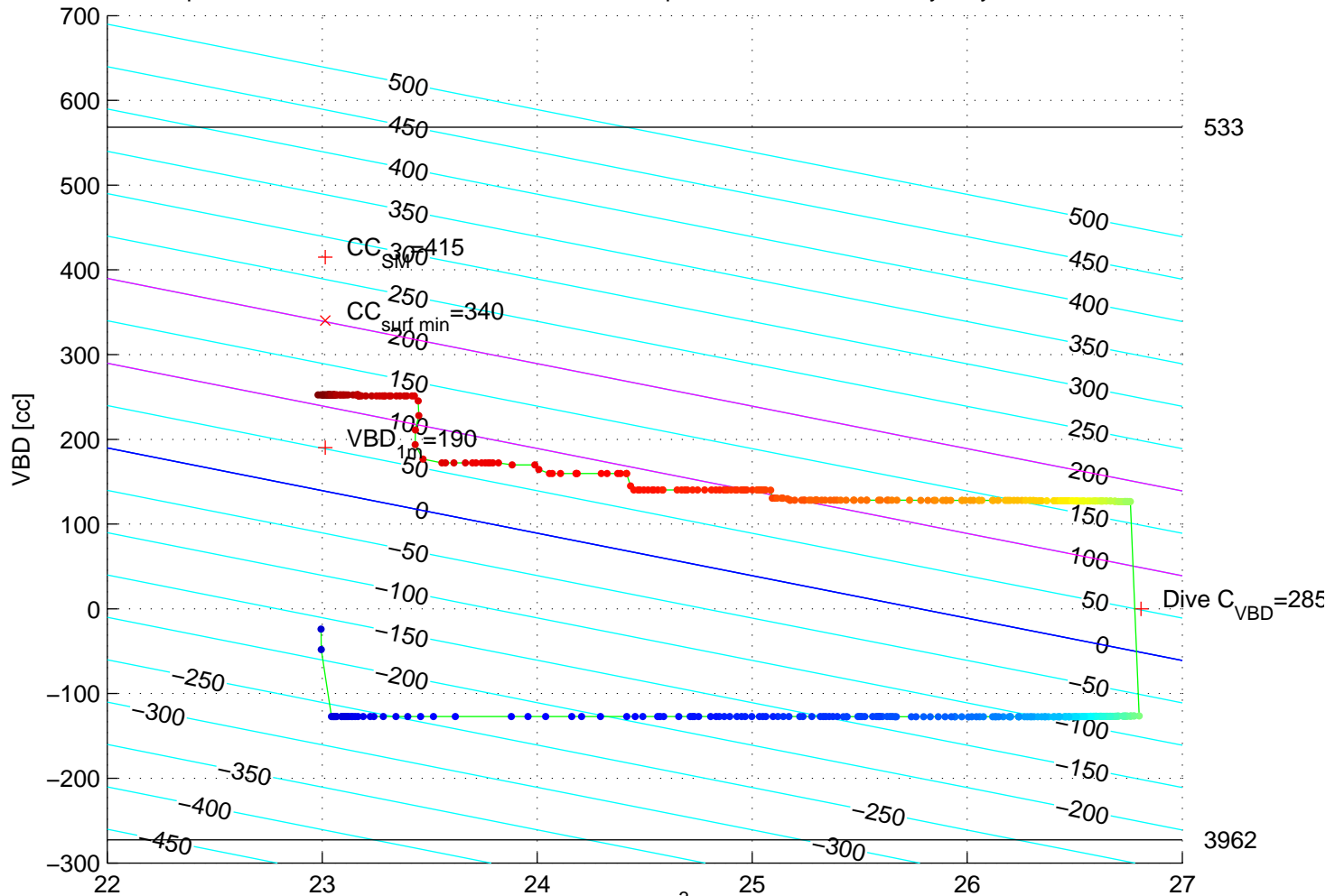
p6350401: SG635 Mission 7 Jul 2017 09-Sep-2017 17:51:52Z - buoyancy contoured
