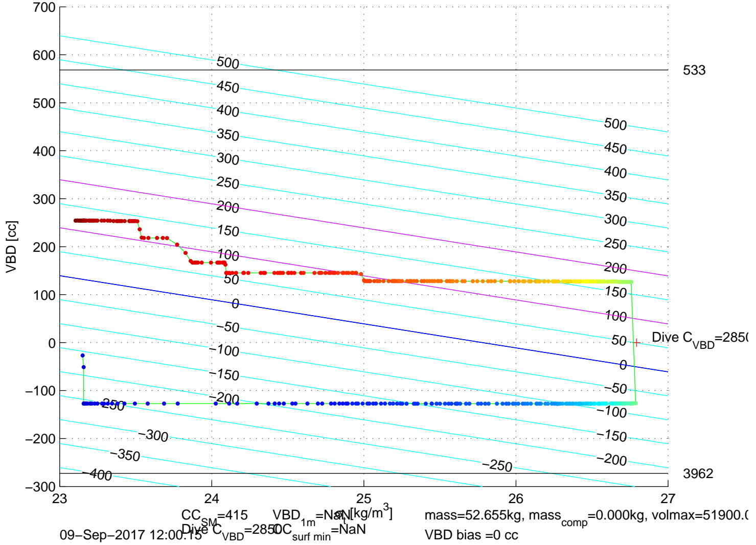
p6350399: SG635 Mission 7 Jul 2017 09-Sep-2017 14:03:10Z - buoyancy contoured
