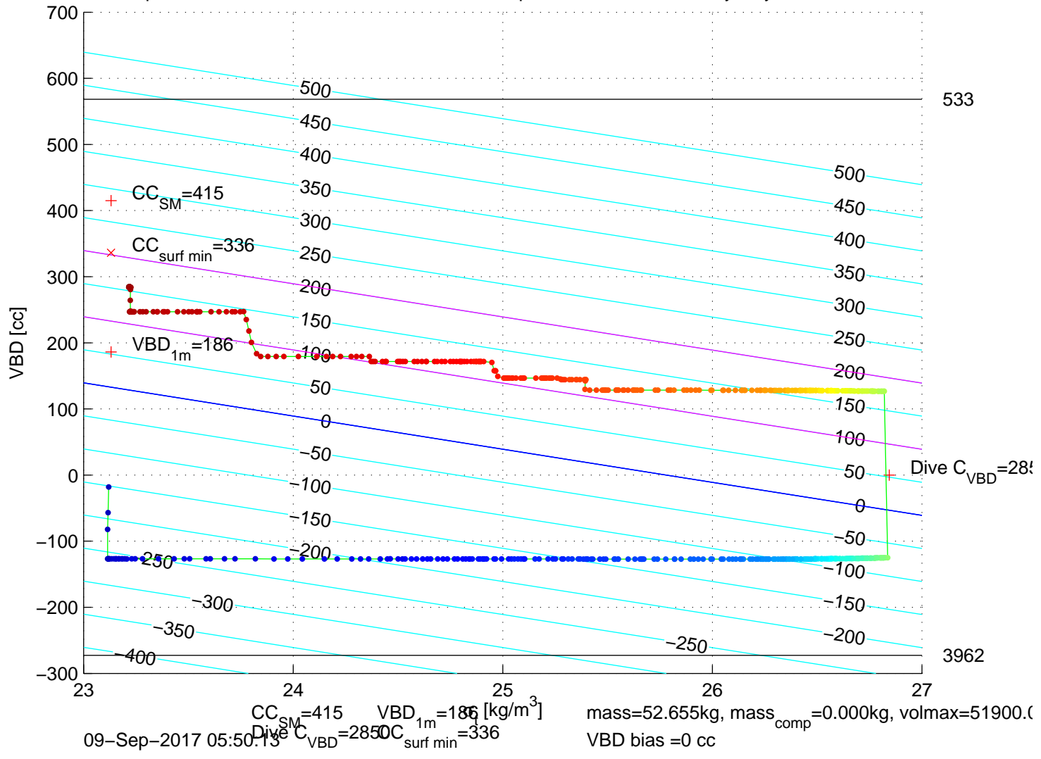
p6350396: SG635 Mission 7 Jul 2017 09-Sep-2017 07:17:04Z - buoyancy contoured
