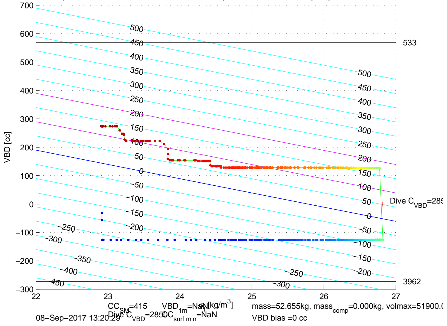
p6350389: SG635 Mission 7 Jul 2017 08-Sep-2017 15:16:40Z – buoyancy contoured
