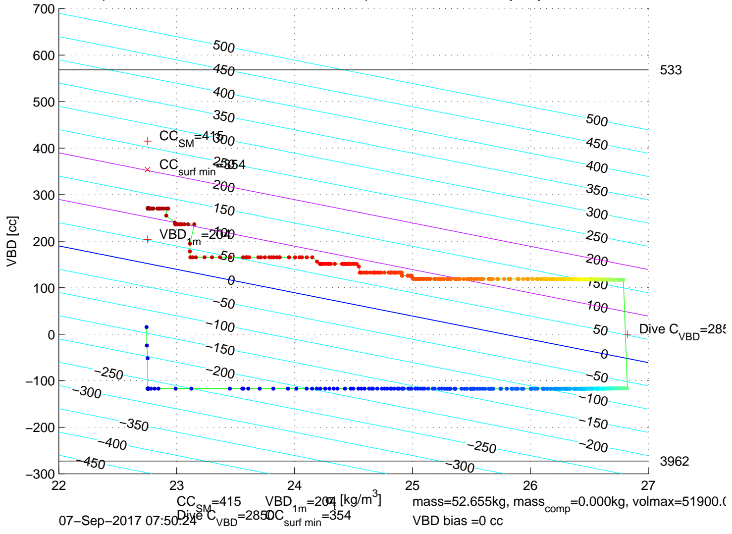
p6350376: SG635 Mission 7 Jul 2017 07-Sep-2017 09:42:14Z – buoyancy contoured
