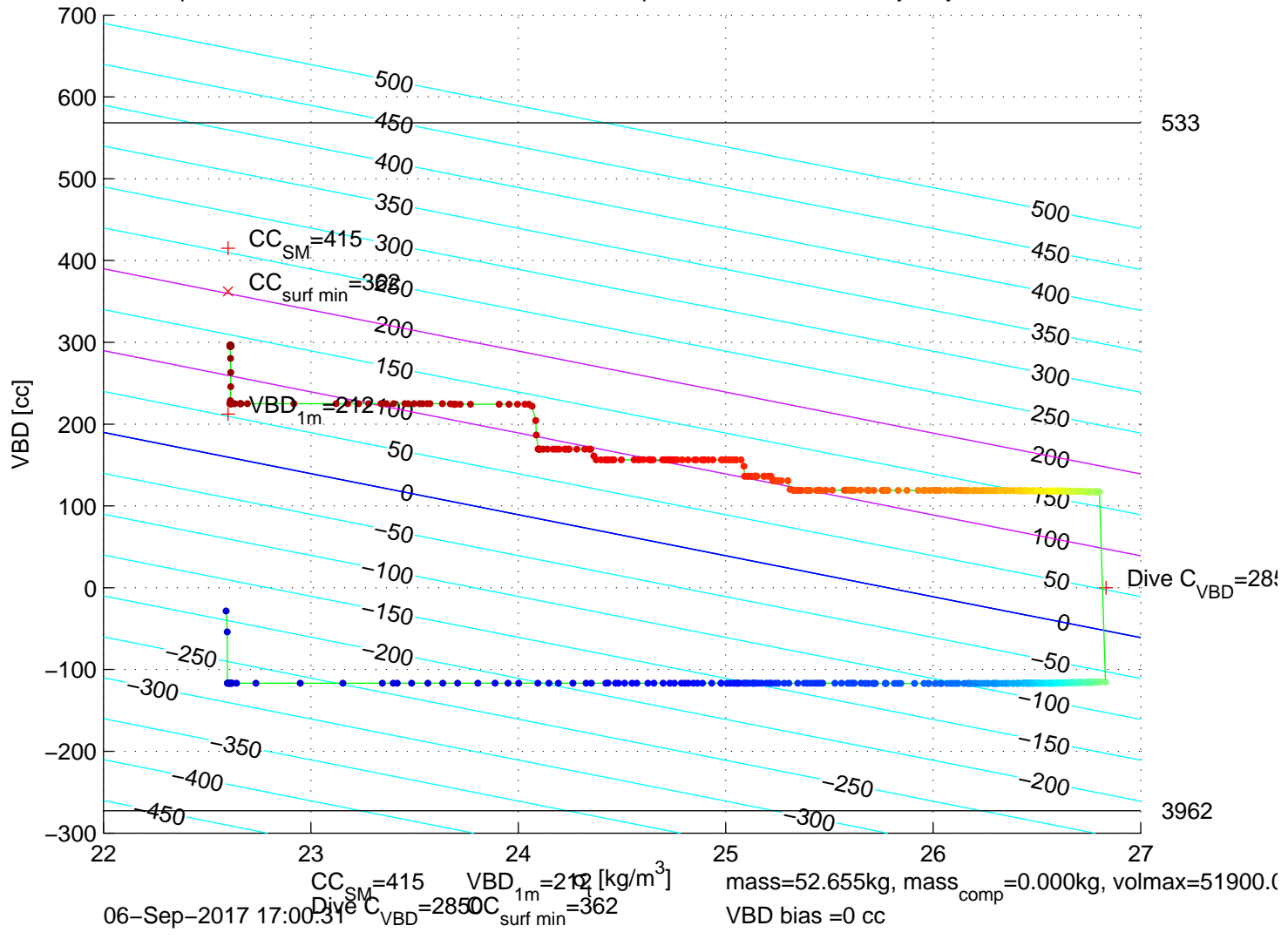
p6350369: SG635 Mission 7 Jul 2017 06–Sep–2017 18:39:24Z – buoyancy contoured
