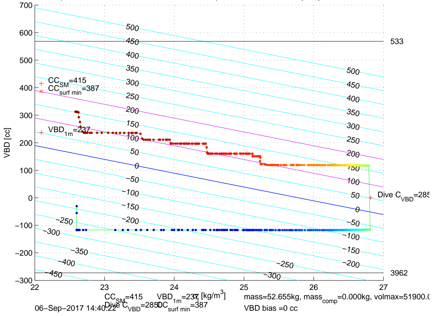
p6350368: SG635 Mission 7 Jul 2017 06-Sep-2017 16:15:15Z – buoyancy contoured
