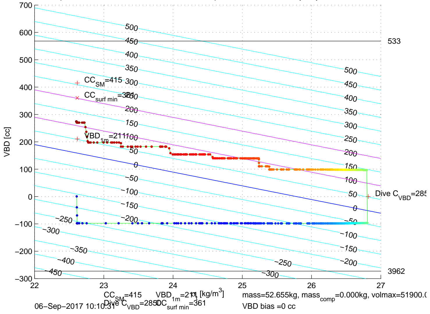
p6350366: SG635 Mission 7 Jul 2017 06-Sep-2017 11:50:23Z – buoyancy contoured
