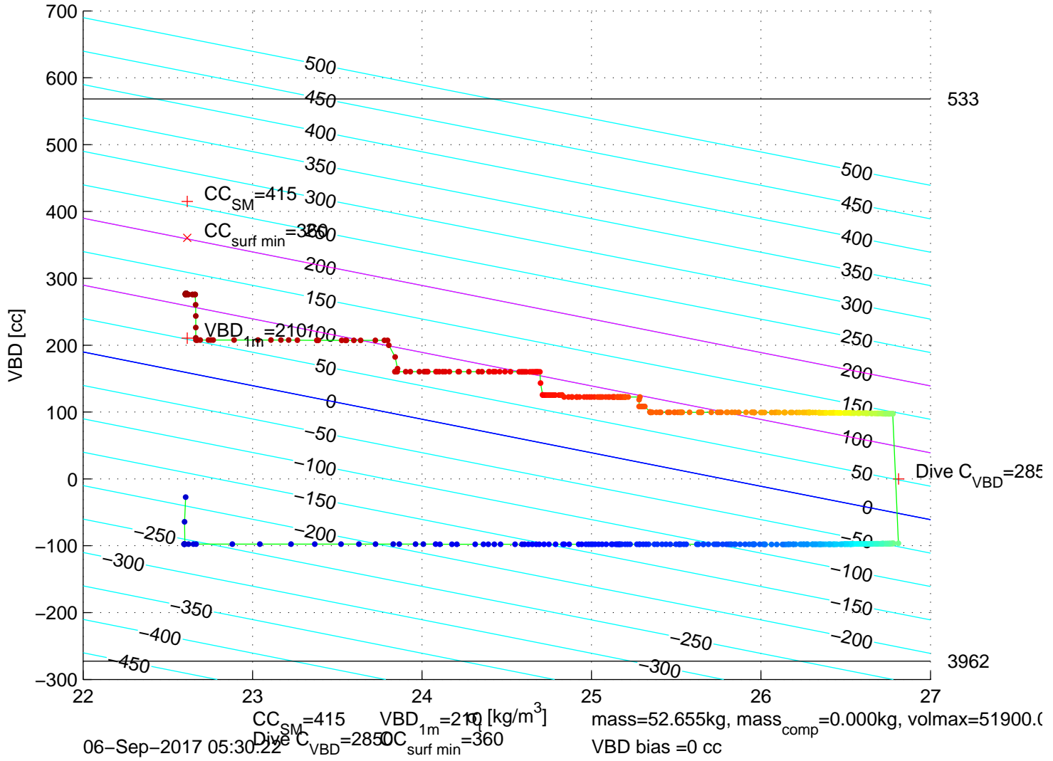
p6350364: SG635 Mission 7 Jul 2017 06-Sep-2017 07:11:35Z – buoyancy contoured
