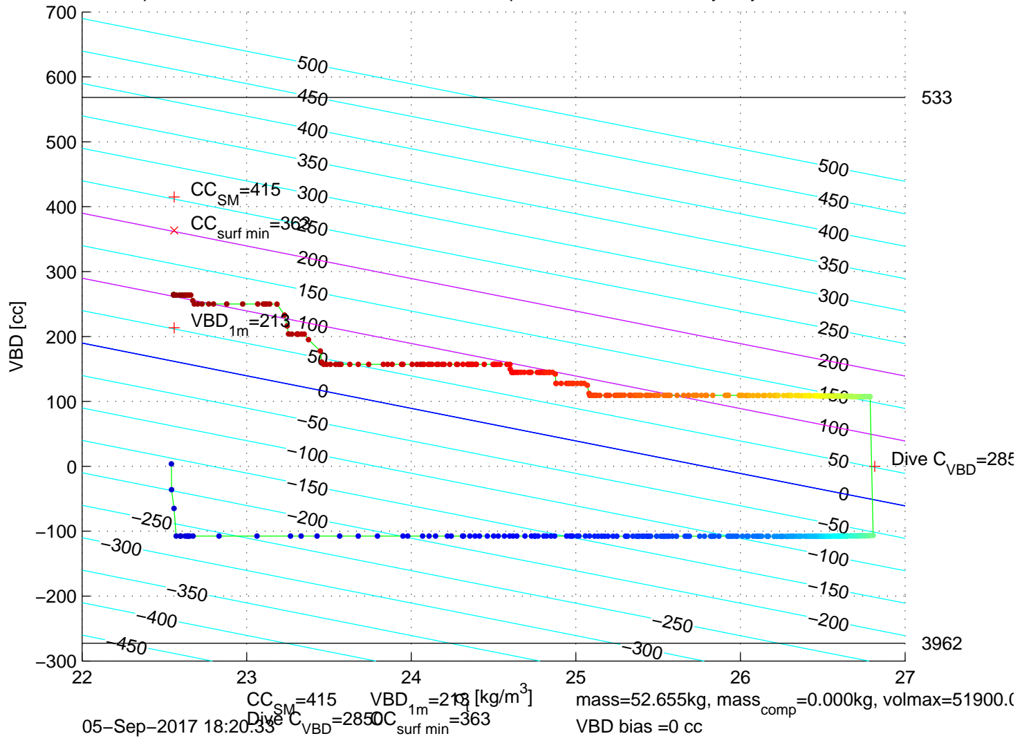
p6350359: SG635 Mission 7 Jul 2017 05-Sep-2017 20:07:45Z – buoyancy contoured
