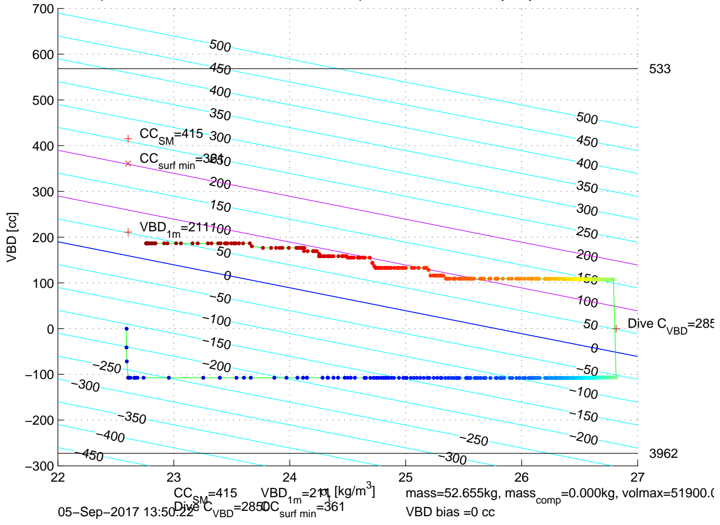
p6350357: SG635 Mission 7 Jul 2017 05-Sep-2017 15:33:36Z – buoyancy contoured
