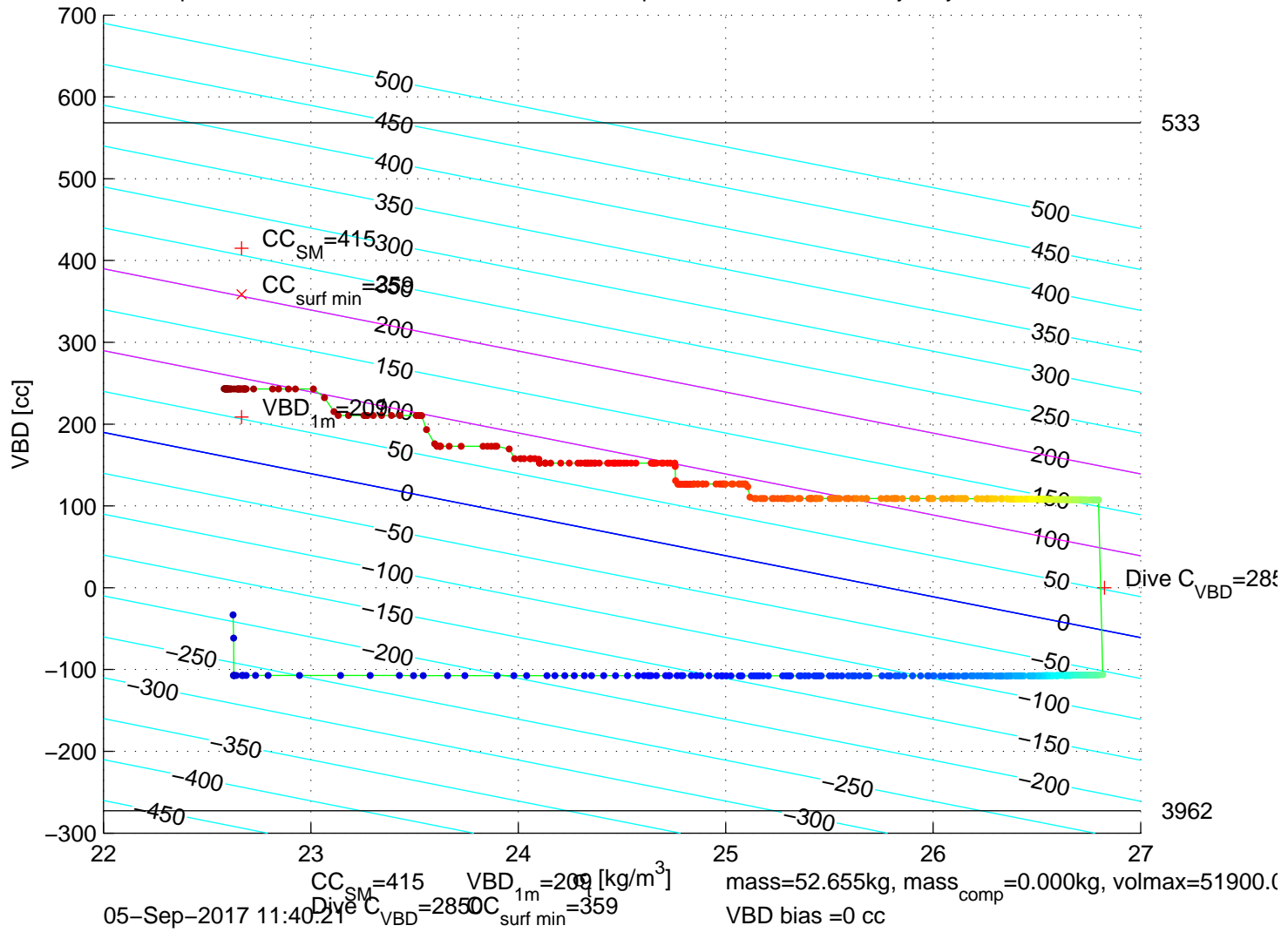
p6350356: SG635 Mission 7 Jul 2017 05-Sep-2017 13:24:49Z – buoyancy contoured
