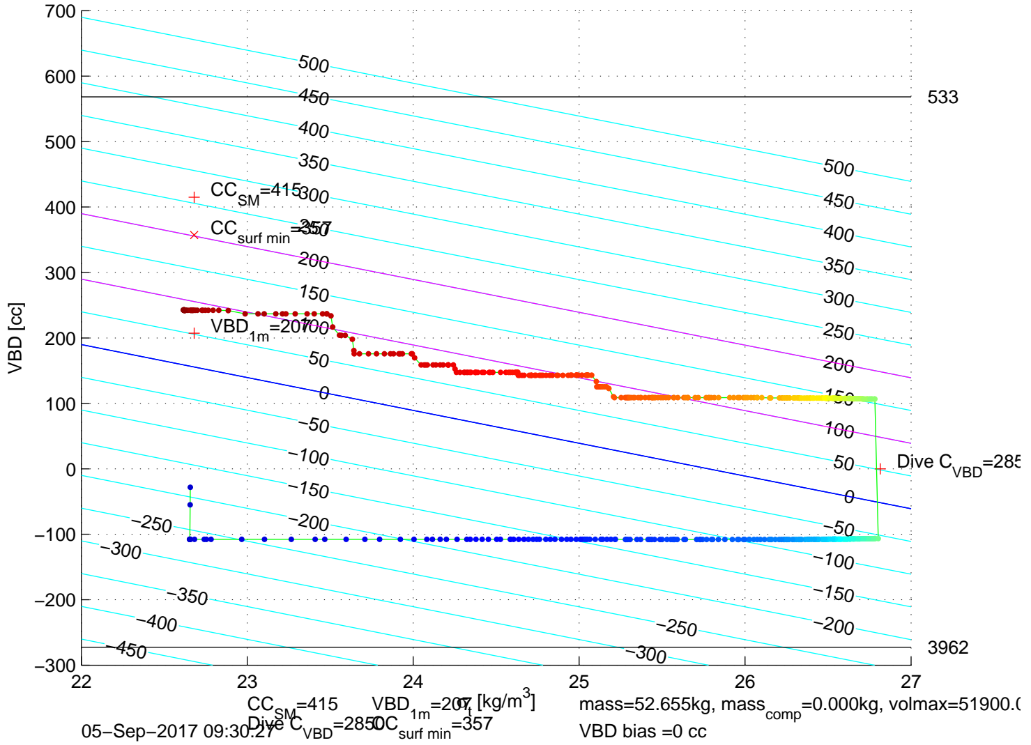
p6350355: SG635 Mission 7 Jul 2017 05-Sep-2017 11:20:06Z – buoyancy contoured
