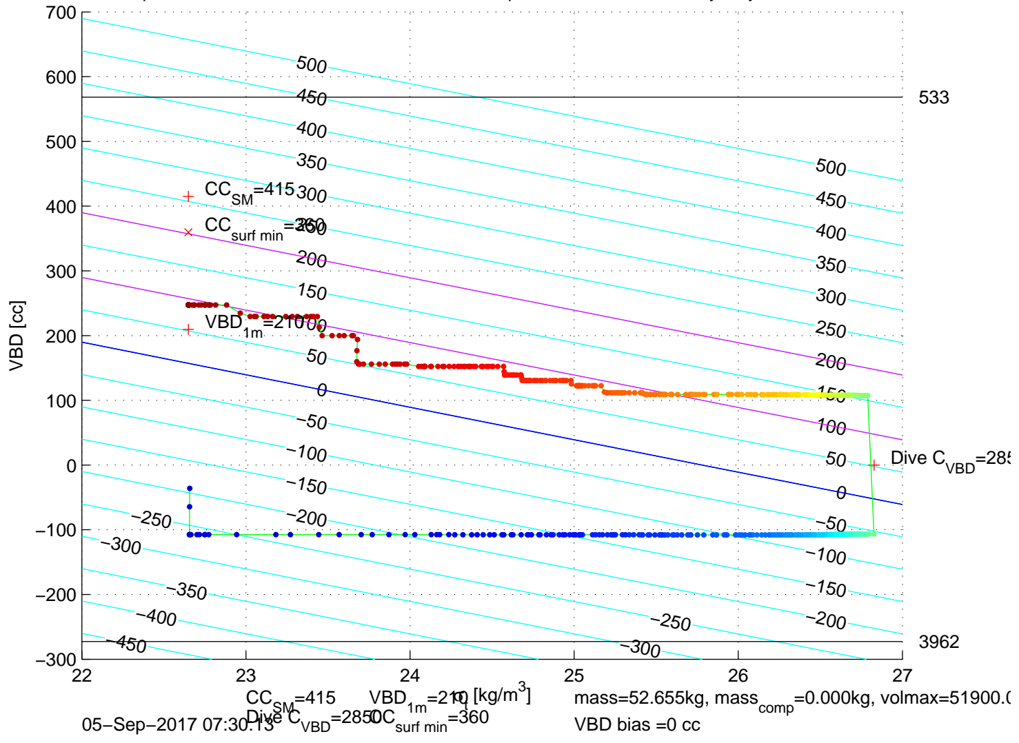
p6350354: SG635 Mission 7 Jul 2017 05-Sep-2017 09:10:41Z – buoyancy contoured
