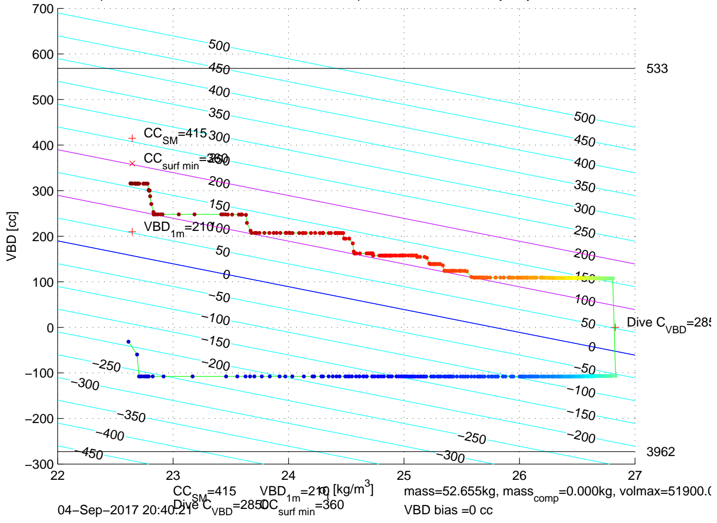
p6350349: SG635 Mission 7 Jul 2017 04-Sep-2017 22:12:25Z – buoyancy contoured
