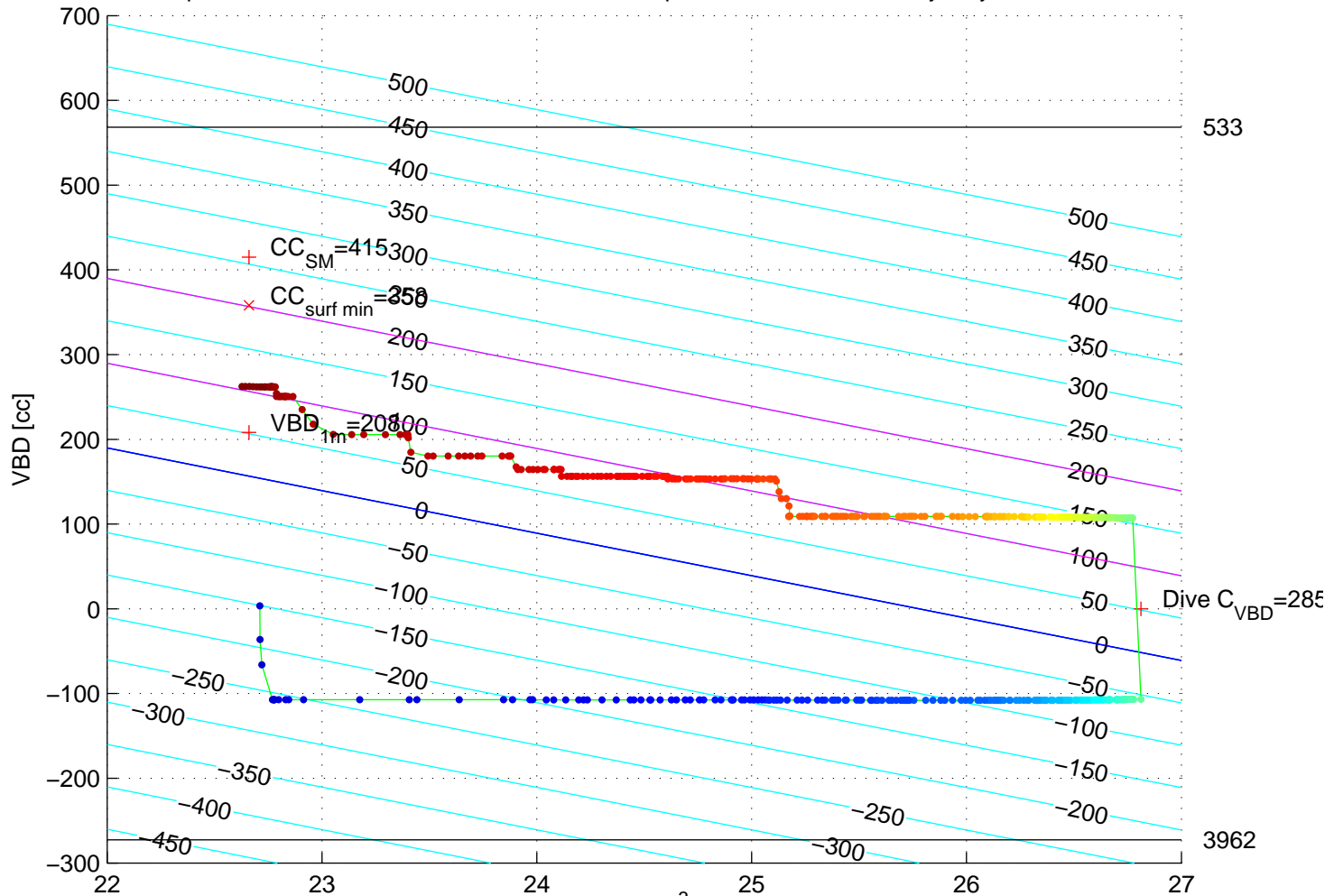
p6350346: SG635 Mission 7 Jul 2017 04-Sep-2017 15:51:53Z – buoyancy contoured
