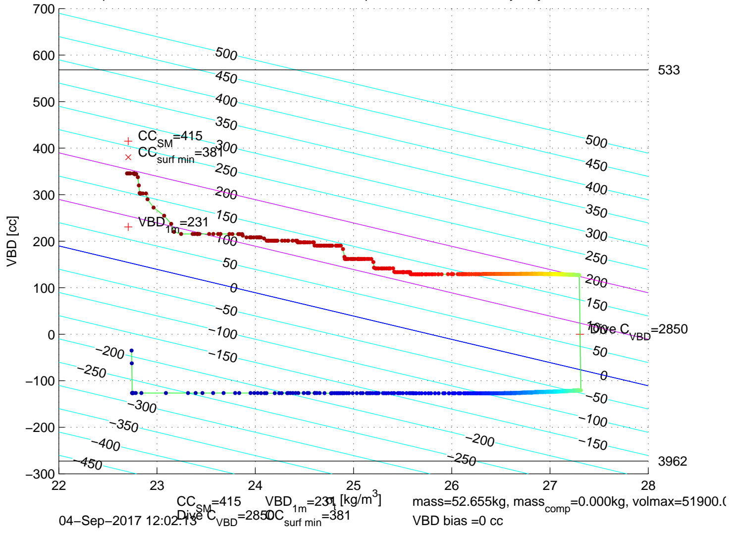
p6350345: SG635 Mission 7 Jul 2017 04-Sep-2017 11:42:24Z – buoyancy contoured
