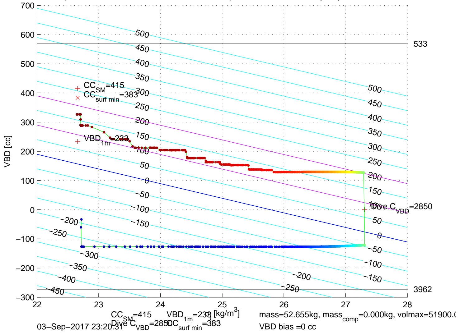
p6350342: SG635 Mission 7 Jul 2017 03-Sep-2017 23:06:17Z – buoyancy contoured
