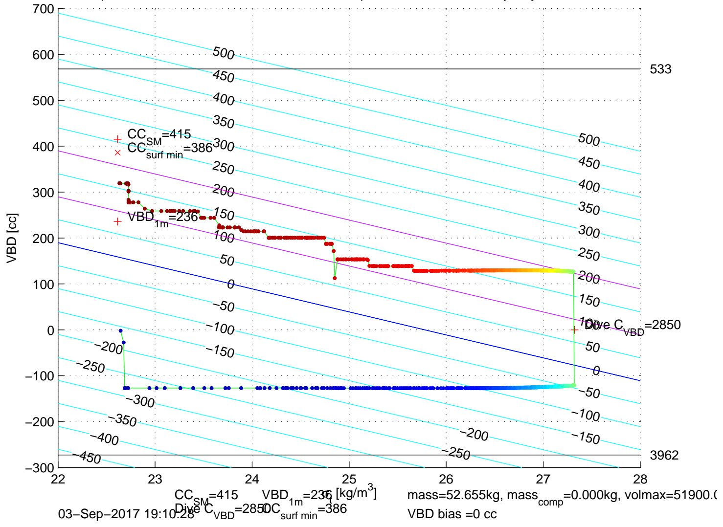
p6350341: SG635 Mission 7 Jul 2017 03-Sep-2017 18:55:37Z – buoyancy contoured
